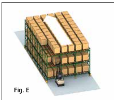
Flow-Thru Rack First-in, first-out Variable truck and aisle
