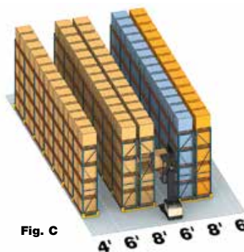
Selective Rack Turret Stockpicker 25% more storage over Fig. B 66% more storage over Fig. A
