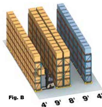
Selective Rack Rider Reach Truck 33% more storage over Fig. A
