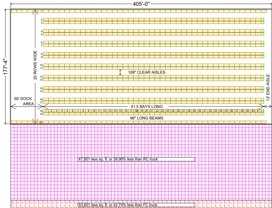
RM - REACH TRUCK LAYOUT 32' CLEAR HEIGHT - 6 PALLETS HIGH, 825 BAYS OF RACK, 9,900 PALLET POSITIONS BUILDING= 71,820 SQUARE FEET, 7.3 SQ. FT. PER PALLET POSITION
